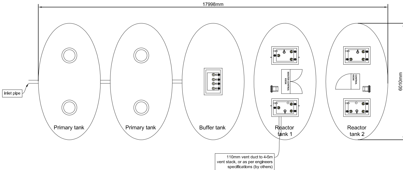
PLAN
