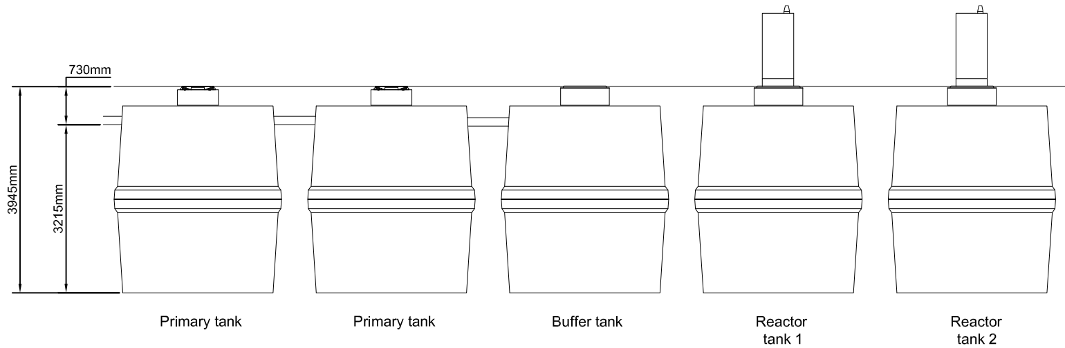
SECTION
