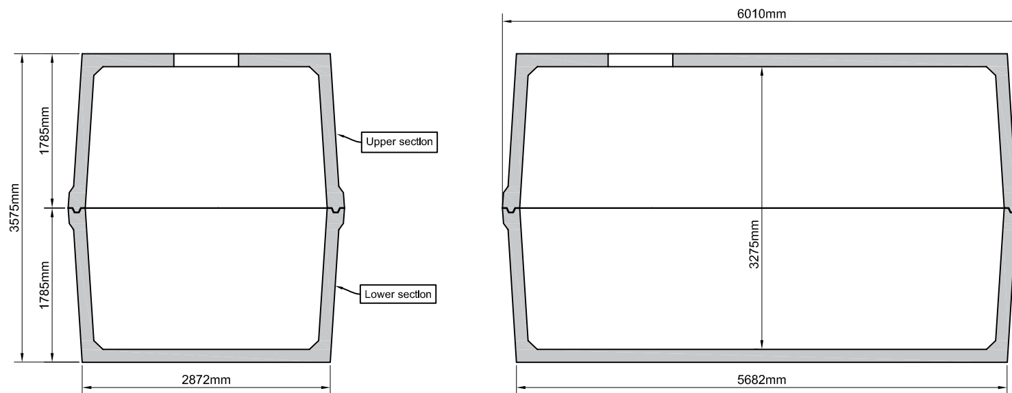
TANK SECTION
