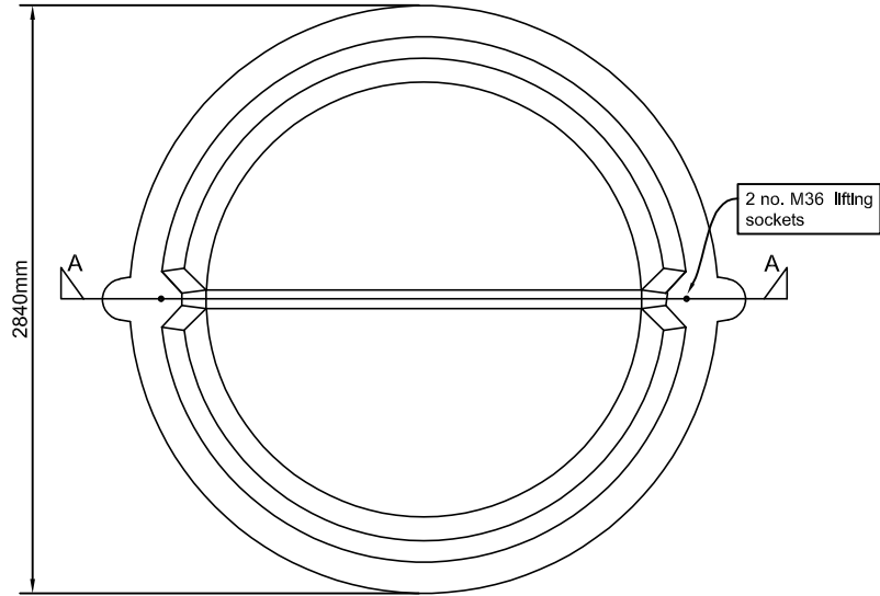
TANK PLAN
