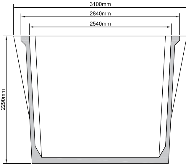
TANK SECTION through A-A
