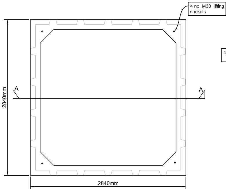
TANK PLAN
