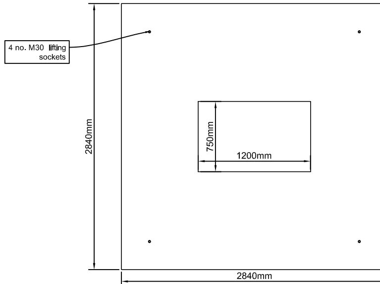
LID PLAN option 1: 1,200 X 750mm opening
