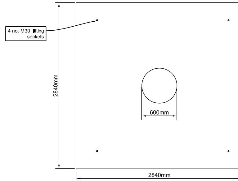
LID PLAN option 2: 600mm opening
