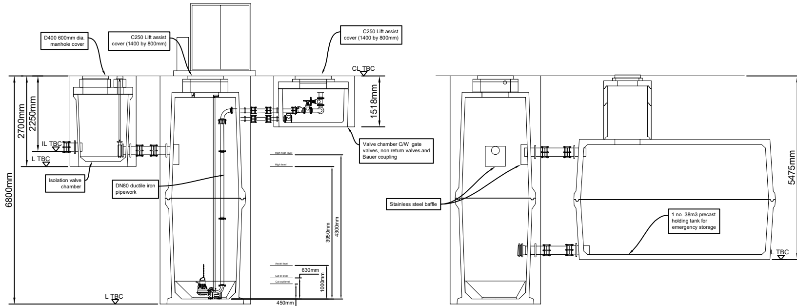
SECTION through A-A
