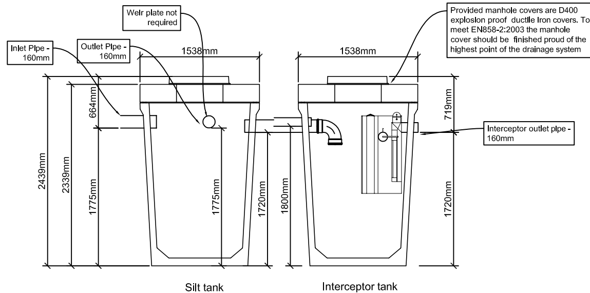
SECTION - Through A-A
