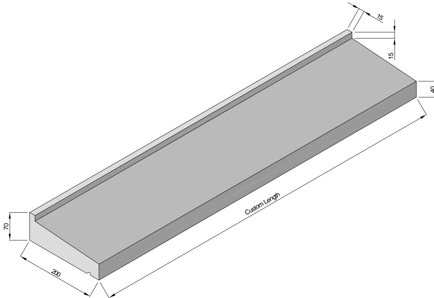
2" Timber Frame Window Cill
